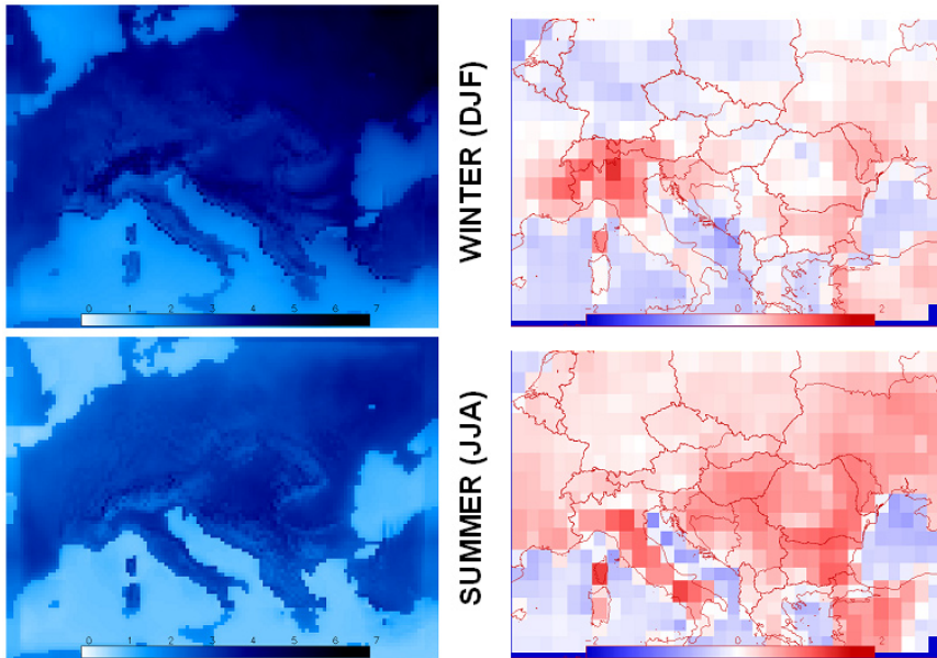
Figure 5. Seasonal standard deviation of temperature ( ^{\circ}\text{C} ) simulations of model PRECIS, and its difference from the standard deviation of ERA40 temperature reanalysis data, 1978–1982
