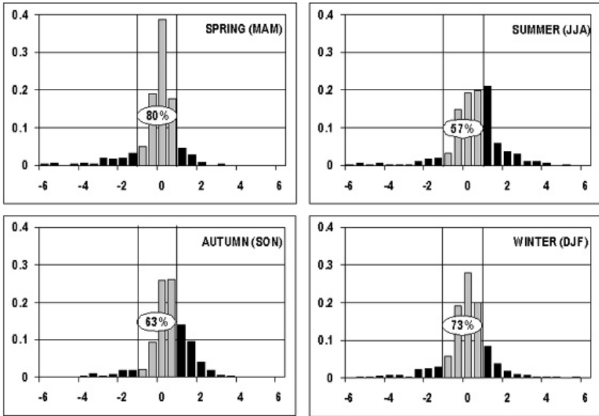
Figure 4. Seasonal distribution of temperature bias (°C) based on simulations of model PRECIS compared to ERA40 reanalysis data, 1978–1982
