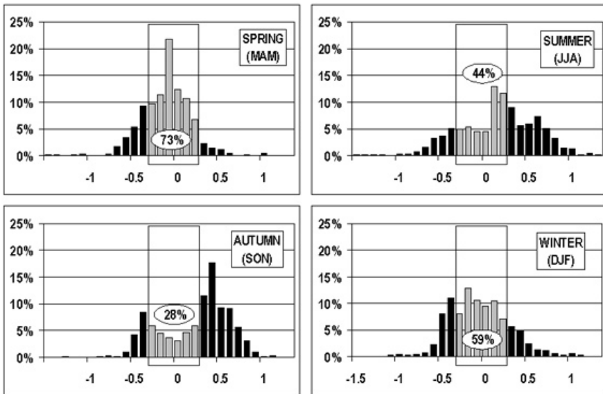
Figure 6. Seasonal distribution of difference between standard deviations of temperature ( ^{\circ}\text{C} ) based on simulations of model PRECIS compared to ERA40 reanalysis data, 1978–1982
