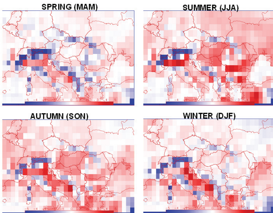
Figure 3. Seasonal temperature bias ( ^\circ \text{C} ) based on simulations of model PRECIS compared to ERA40 reanalysis data, 1978–1982
