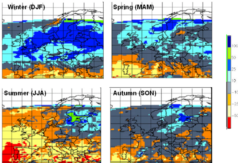
Figure 2. Seasonal precipitation change (%) based on climate projections of model RegCM (ICTP) in case of scenario SRES A2, 2071–2100
