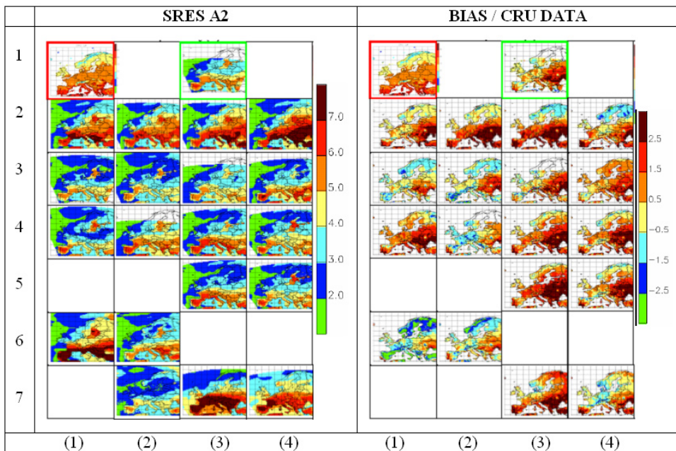
Figure 1. Mean temperature change (°C) in summer in case of 19 models: projections for scenario SRES A2 (left), difference between the simulated and CRU data for present climate (right). Maps are ordered as follows: Models in Row 1: (1) CRU control, (3) average of all model simulations; Models in Row 2: (1) HadAM3H, (2) HadRM3H, (3) HadRM3P, (4) HadAM3P – Britain; Models in Row 3: (1) ETH – Switzerland, (2) GKSS – Germany, (3) ICTP – Italy, (4) KNMI – Netherlands; Models in Row 4: (1) MPI – Germany, (2) UCM – Britain, (3) SMHI – Sweden, (4) DMI – Denmark; Models in Row 5: (3) SMHI (22 km resolution) – Sweden, (4) DMI (25 km resolution) – Denmark; Models in Row 6: (1) HadCM3 – Britain, (2) CNRM – France; Models in Row 7: (2) CNRM/A – France, (3) SMHI/E – Sweden, (4) DMI/E – Denmark. (Source: Christensen, 2005)
